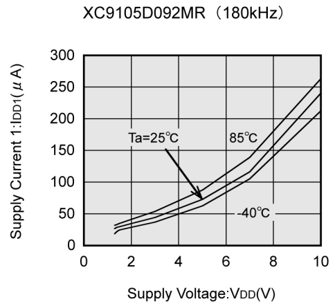
(5) Supply Current 1 vs. Power Supply Voltage
